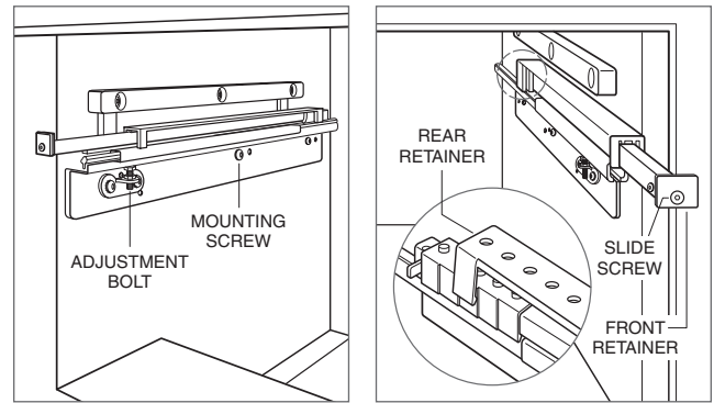
Vertical adjustment.
