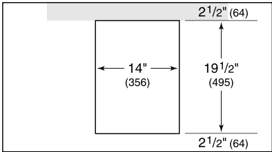
COUNTERTOP CUT-OUT
