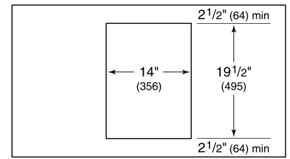
COUNTERTOP CUT-OUT
